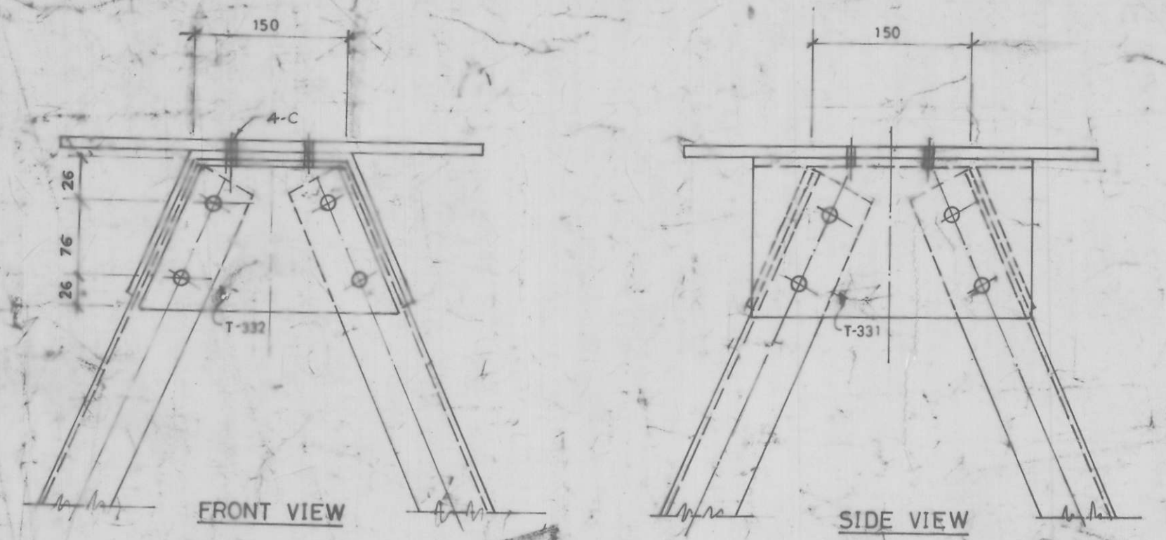
DETAIL AT 'A'
